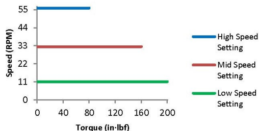
110558 PowerCube™ Assembly 10:1 Reducer, 200W Motor, 110546 Control
