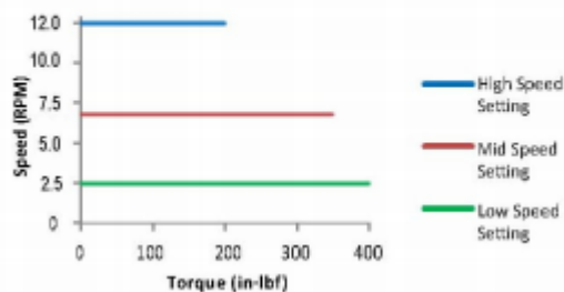
110216 PowerCube™ Assembly 30:1 Reducer, 125W Motor, 110546 Control
